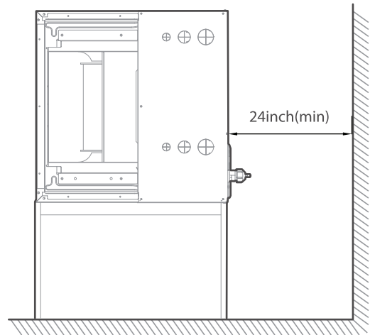
Installations horizontales
