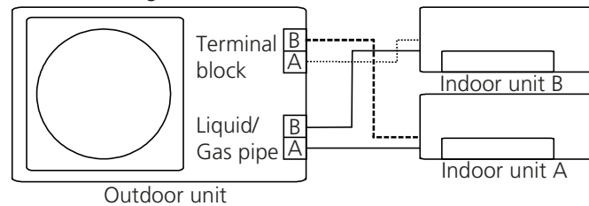
Incorrect wiring
