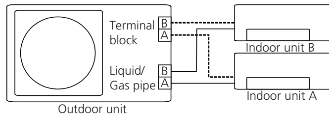
Incorrect wiring
