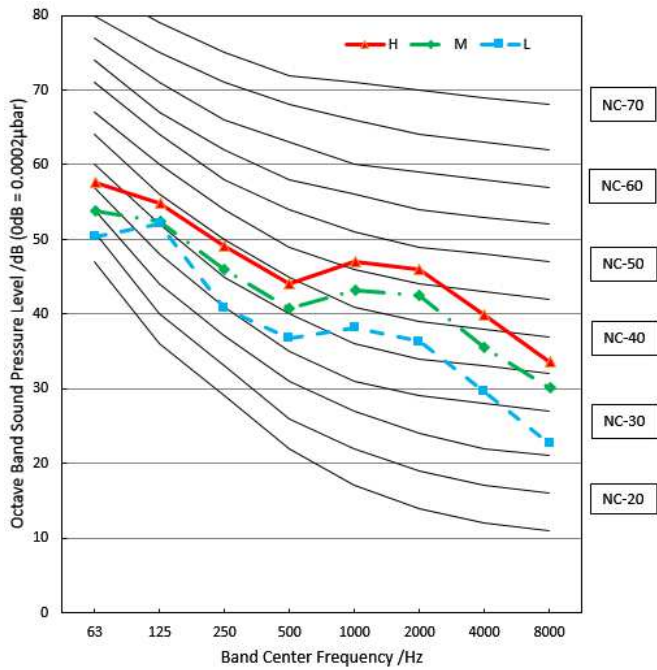
MVC-48HWFN1-M
