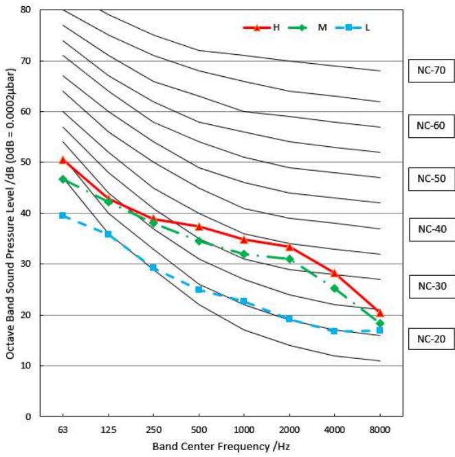
MVC-48HWFN1-M
