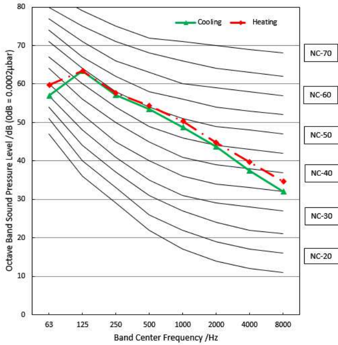
MOD30U-30HFN1-MR0(X)
